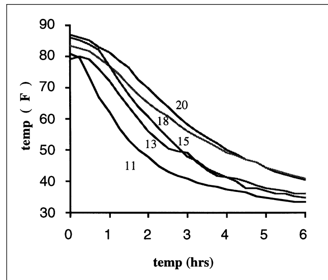
Figure 4. Chill curves of fish cooled in slush ice. The different curves represent fish of different weights, in pounds.
