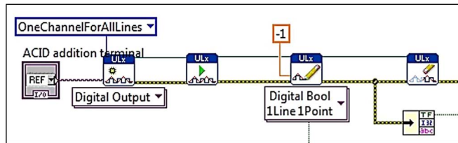
Fig. 4.1. Section 1 from Fig. 4 expanded to show programmatic detail. Depicts graphical code for connecting the MC control board to the pHstat system.
