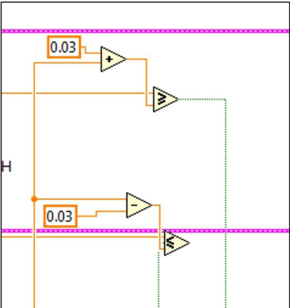
Fig. 3.4. Section 4 from Fig. 3 expanded to show programmatic detail. Depicts programmatic element of pH control using Boolean operators to maintain pH thresholds within a set pH points of the guide pH at any given time.
