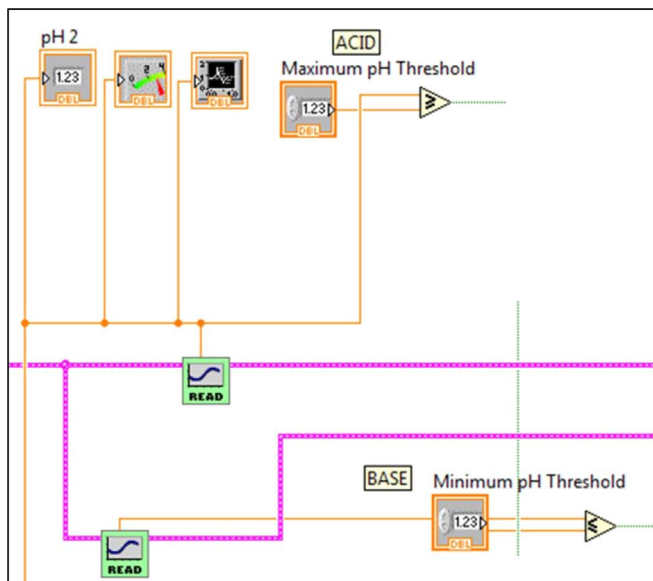
Fig. 4.2. Section 2 from Fig. 4 expanded to show programmatic detail. Depicts programmatic element of pH control using front panel indicators to maintain pH within thresholds. Broken wires connect to other elements, which were deleted for clarity.
