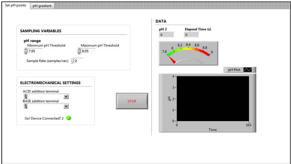
Fig. 1. Front panel of virtual instrument (VI) for producing a steady state pH environment.
