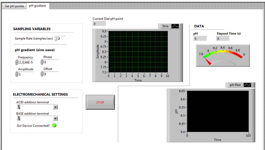
Fig. 2. Front panel of virtual instrument (VI) for producing a dynamic pH environment based on a sine wave.
