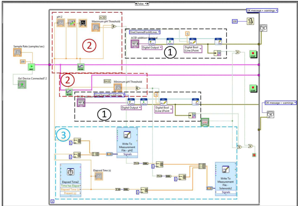
Fig. 4. Block diagram for VI showing graphical code for steady state pH functionality. Sections 1, 2, and 3 match up to Figs. 4.1, 4.2, and 4.3, respectively.
