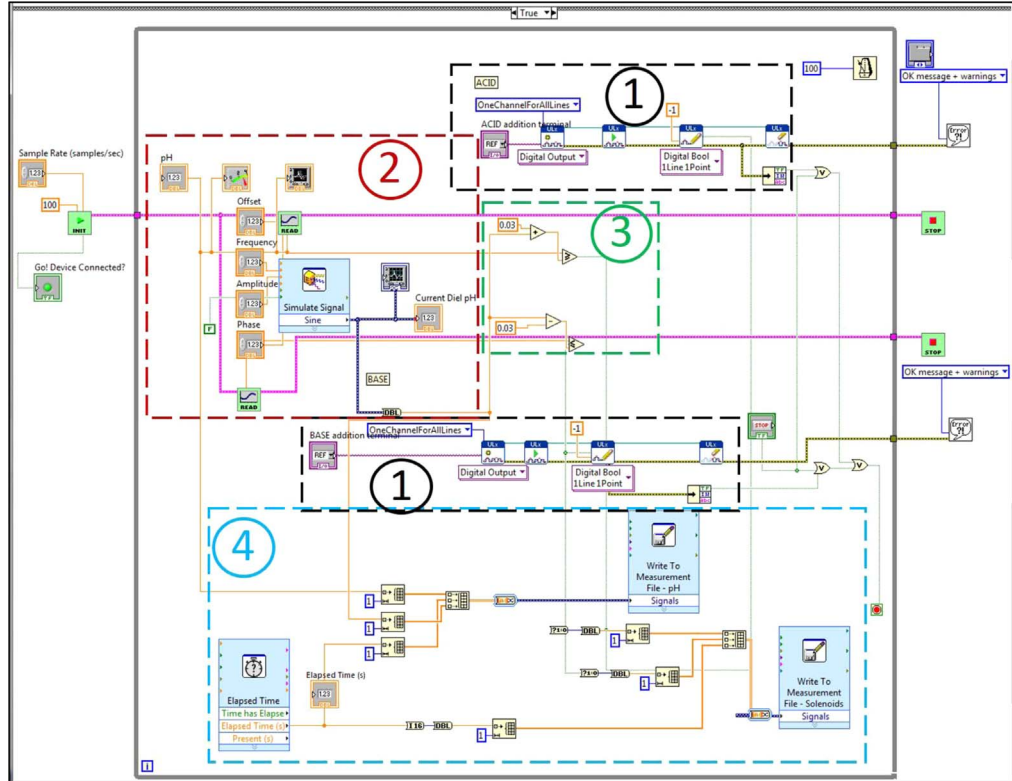
Fig. 3. Block diagram for VI showing graphical code for dynamic pH functionality. Sections 1, 2, 3, and 4 correspond to Figs. 3.1, 3.2, 3.3, and 3.4, respectively.
