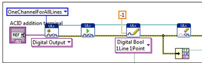
Fig. 3.1. Section 1 from Fig. 3 expanded to show programmatic detail. Depicts graphical code for connecting the MC control board to the pHstat system.
