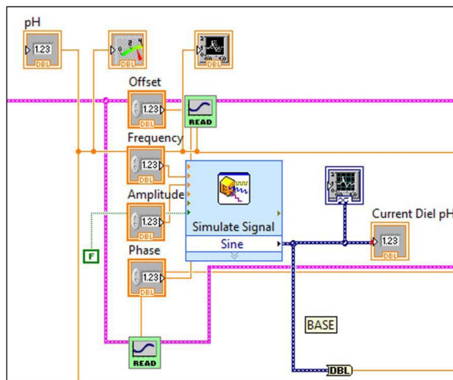
Fig. 3.3. Section 3 from Fig. 3 expanded to show programmatic detail. Shows subVI for providing the guide pH for the dynamic functionality of the pHStat. Guide pH is generated using a sine wave, with the user setting the frequency, offset, amplitude, and phase in order to time the wave to start at a desired pH. Details on how the dynamic functionality works can be found in Golda et al. [2].
